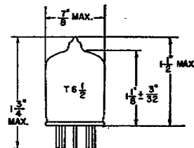
RETMA 4-1
