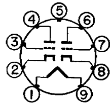
RETMA 8CJ
